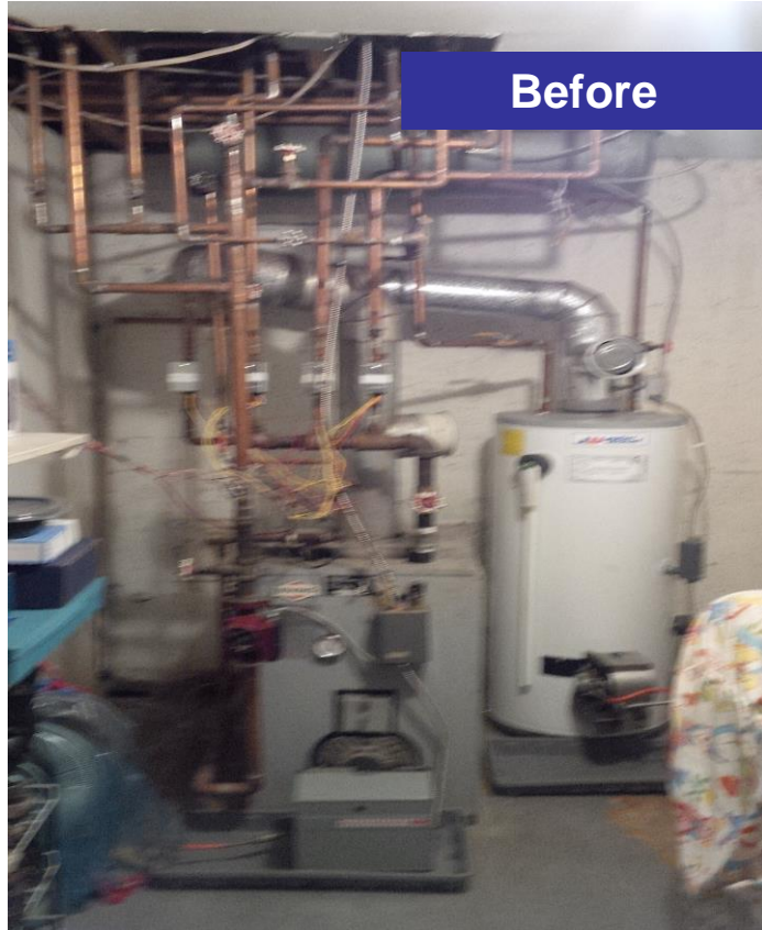
Oil boiler with oil water heater
