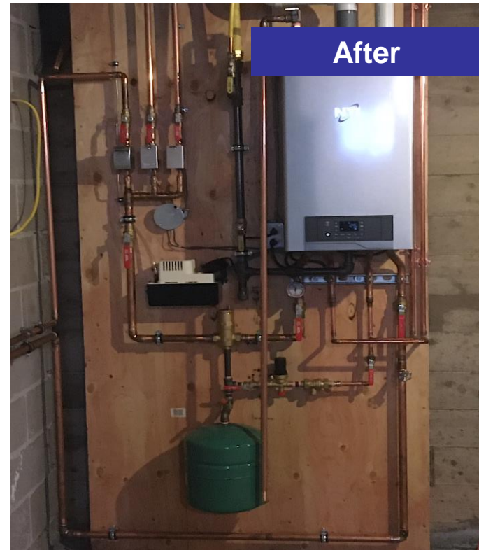
Propane boiler with tankless water heater built in
