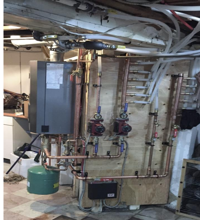
Propane boiler with tankless water heater built in
